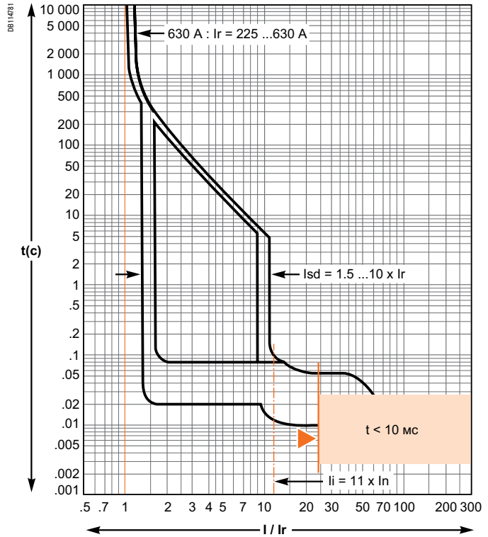
Micrologic 2.3 - 630 А
