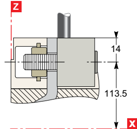
NSX400/630
