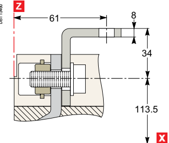
NSX400/630
