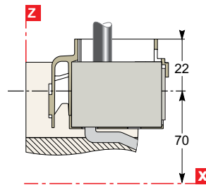
NSX400/630
